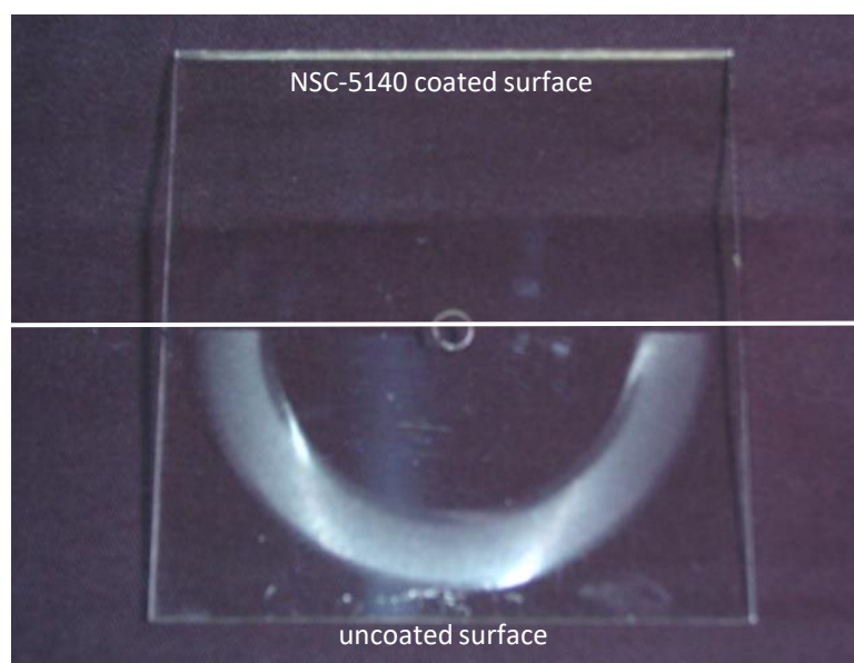
Taber abrasion test CS-10F 500g load \times 100 rotations
